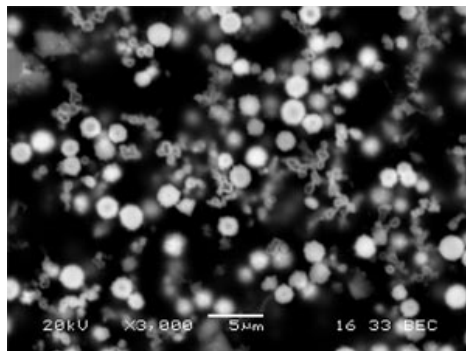
Figure 2 SEM image of micro hematite in synthetic Martian soil.
