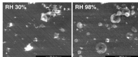
Figure 1 Formation of water droplets in ESEM chamber
