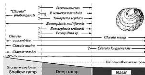
Figure 2 Reconstructed habitats of the Lower Triassic bivalves.
